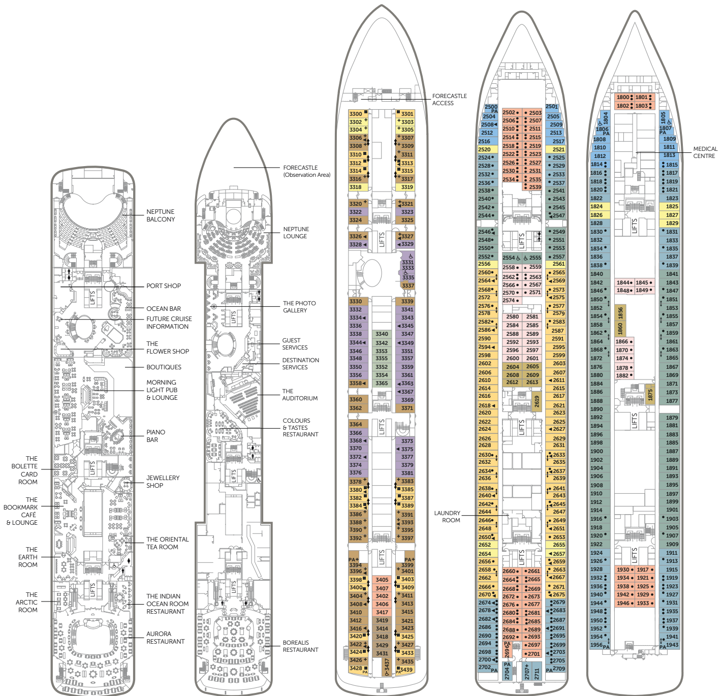
Lounge Deck 5
